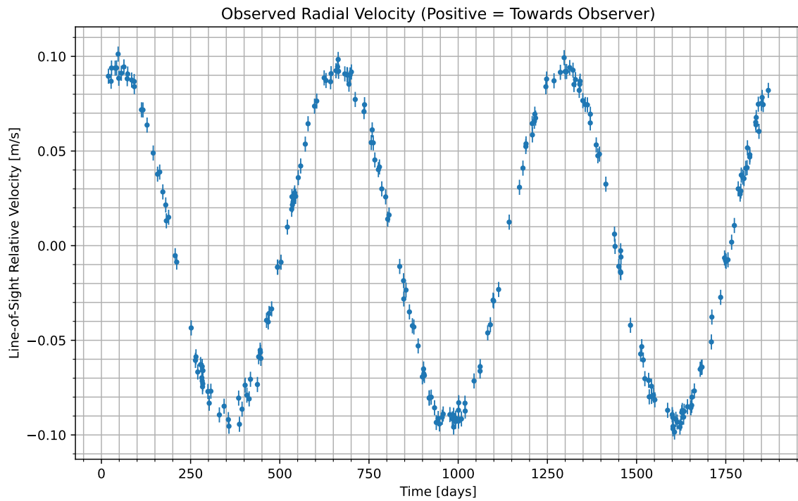
Figure 1: We have isolated the radial velocity of the host star due to the candidate planet. Data begins at UTC 2069-11-09/03:25. Positive values indicate the velocity at which the star is moving towards us; negative indicate the velocity at which it is moving away.
