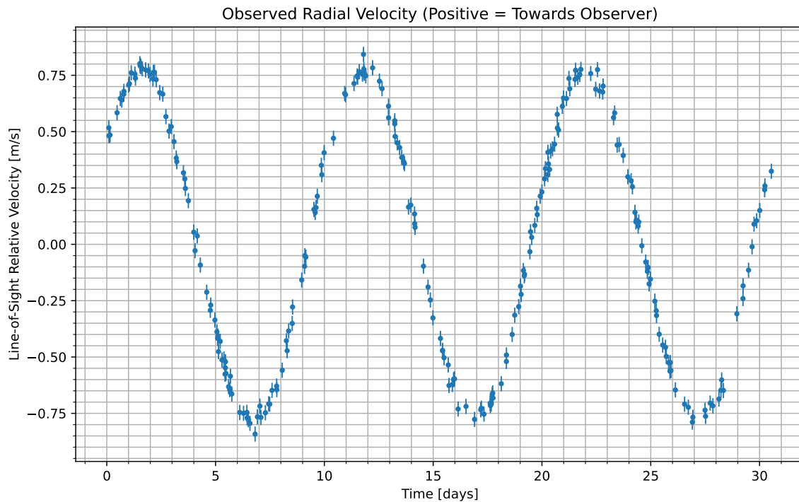
Figure 1: We have isolated the radial velocity of the host star due to the candidate planet. Data begins at UTC 2083-07-11/12:27. Positive values indicate the velocity at which the star is moving towards us; negative indicate the velocity at which it is moving away.
