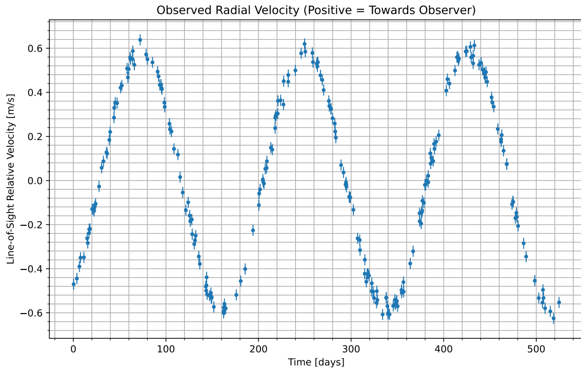
Figure 1: We have isolated the radial velocity of the host star due to the candidate planet. Data begins at UTC 2088-03-12/03:09. Positive values indicate the velocity at which the star is moving towards us; negative indicate the velocity at which it is moving away.
