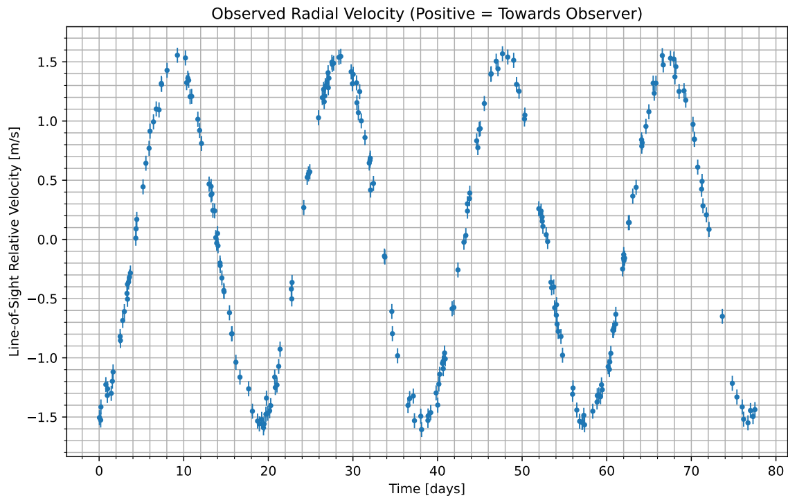
Figure 1: We have isolated the radial velocity of the host star due to the candidate planet. Data begins at UTC 2077-07-02/00:10. Positive values indicate the velocity at which the star is moving towards us; negative indicate the velocity at which it is moving away.
