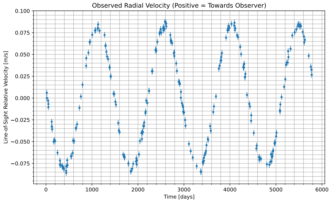
Figure 1: We have isolated the radial velocity of the host star due to the candidate planet. Data begins at UTC 2076-03-13/17:32. Positive values indicate the velocity at which the star is moving towards us; negative indicate the velocity at which it is moving away.
