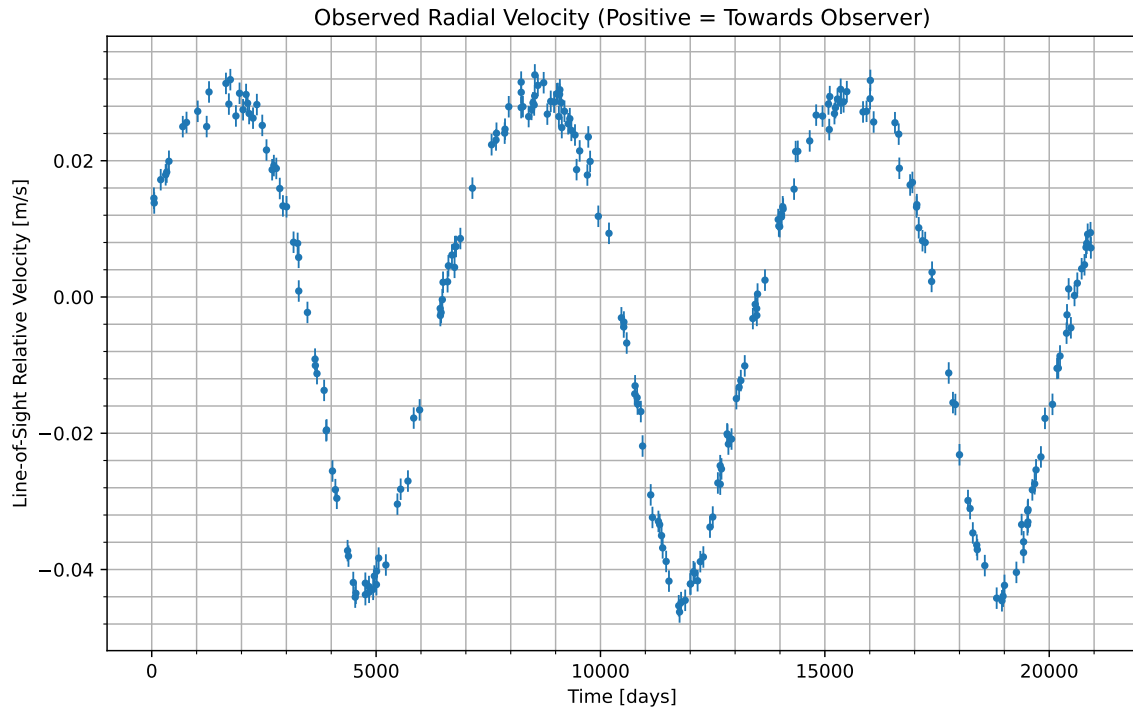
Figure 1: We have isolated the radial velocity of the host star due to the candidate planet. Data begins at UTC 2022-08-21/05:27. Positive values indicate the velocity at which the star is moving towards us; negative indicate the velocity at which it is moving away.
