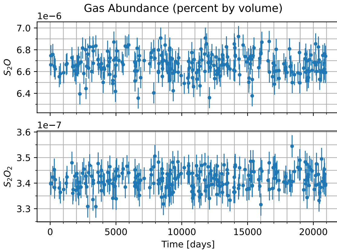
Figure 4: Concentration of various additional gases in the atmosphere of the candidate planet versus time. Note that the y-axis will usually only show the variation multiplied by some factor, shown in the upper left, and then added to some normal amount, also in the upper-left.
