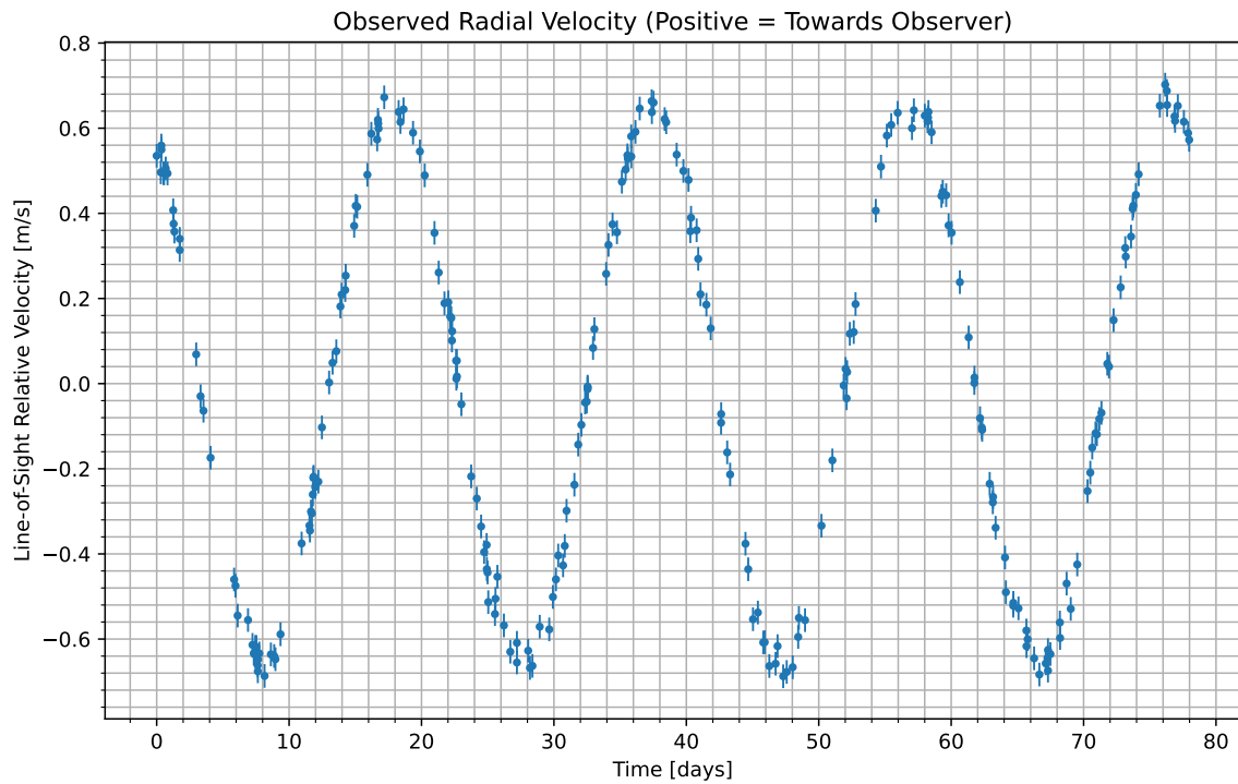
Figure 1: We have isolated the radial velocity of the host star due to the candidate planet. Data begins at UTC 2071-09-18/20:08. Positive values indicate the velocity at which the star is moving towards us; negative indicate the velocity at which it is moving away.
