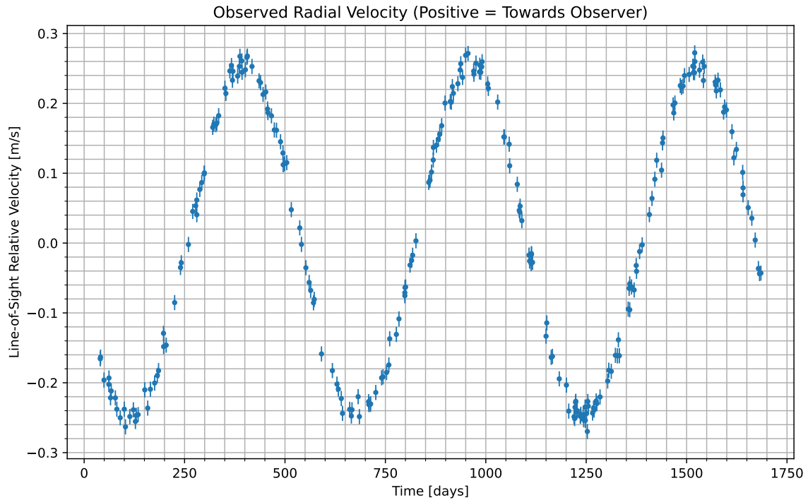
Figure 1: We have isolated the radial velocity of the host star due to the candidate planet. Data begins at UTC 2078-04-12/12:25. Positive values indicate the velocity at which the star is moving towards us; negative indicate the velocity at which it is moving away.
