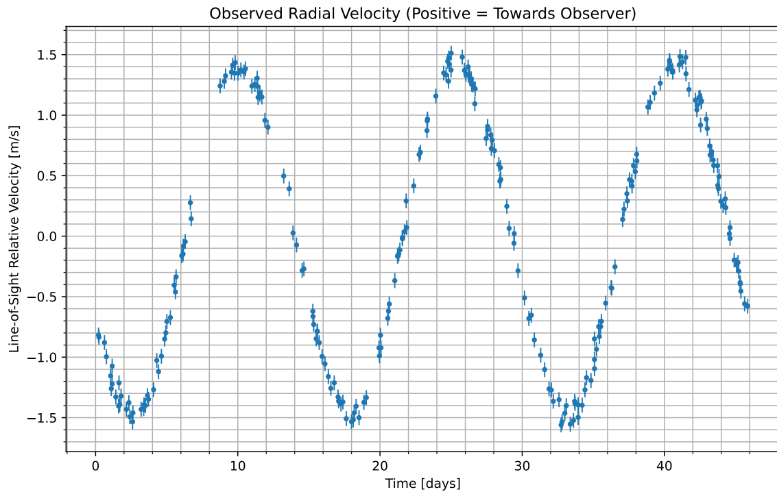
Figure 1: We have isolated the radial velocity of the host star due to the candidate planet. Data begins at UTC 2072-12-23/22:01. Positive values indicate the velocity at which the star is moving towards us; negative indicate the velocity at which it is moving away.
