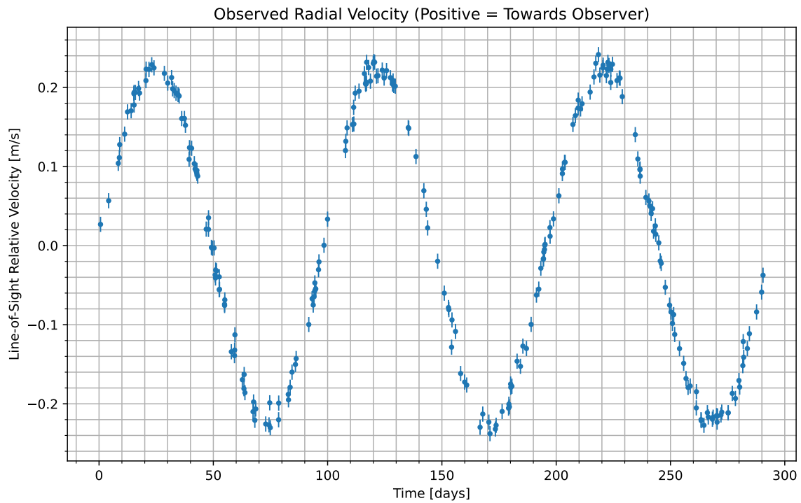
Figure 1: We have isolated the radial velocity of the host star due to the candidate planet. Data begins at UTC 2081-02-07/06:19. Positive values indicate the velocity at which the star is moving towards us; negative indicate the velocity at which it is moving away.
