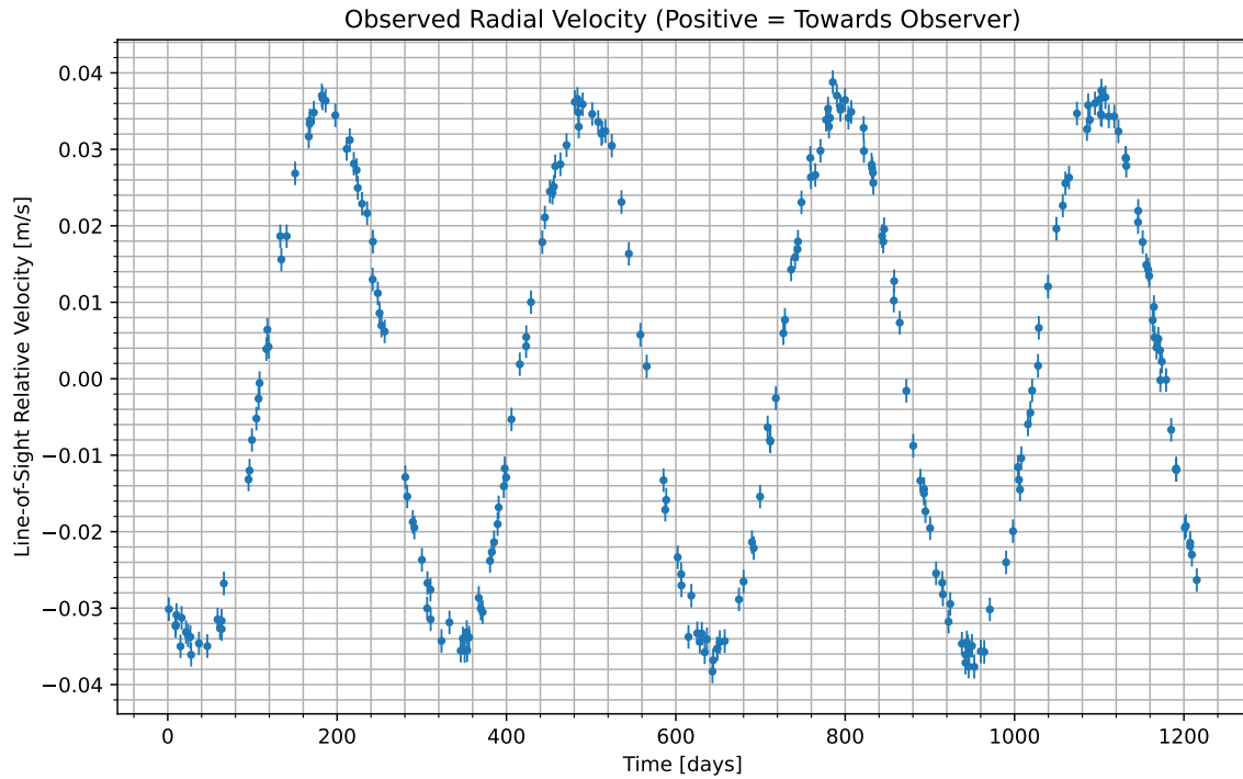
Figure 1: We have isolated the radial velocity of the host star due to the candidate planet. Data begins at UTC 2075-03-07/17:19. Positive values indicate the velocity at which the star is moving towards us; negative indicate the velocity at which it is moving away.
