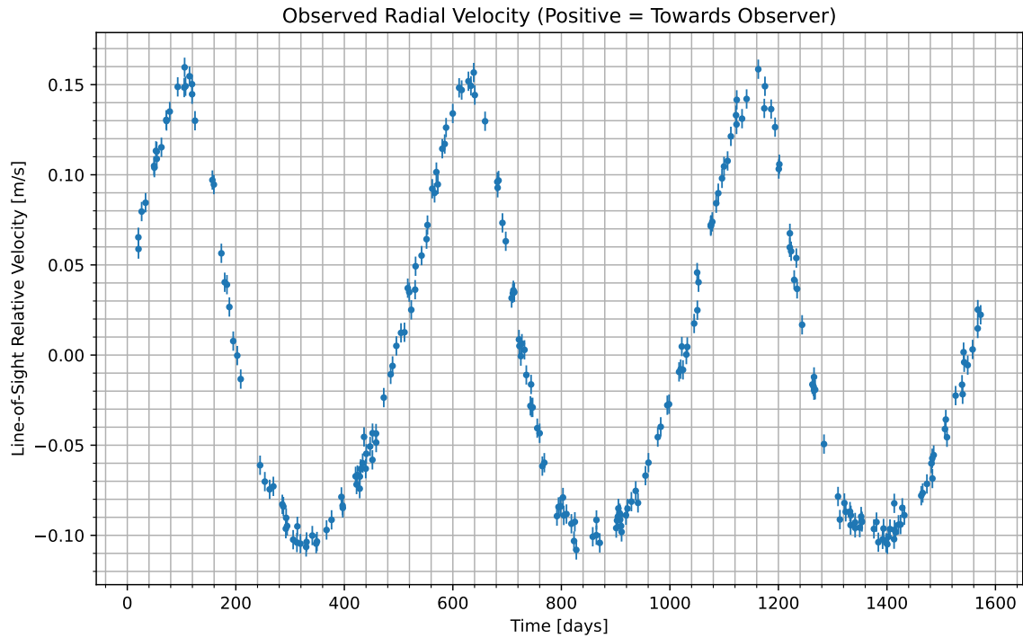
Figure 1: We have isolated the radial velocity of the host star due to the candidate planet. Data begins at UTC 2076-12-24/04:02. Positive values indicate the velocity at which the star is moving towards us; negative indicate the velocity at which it is moving away.
