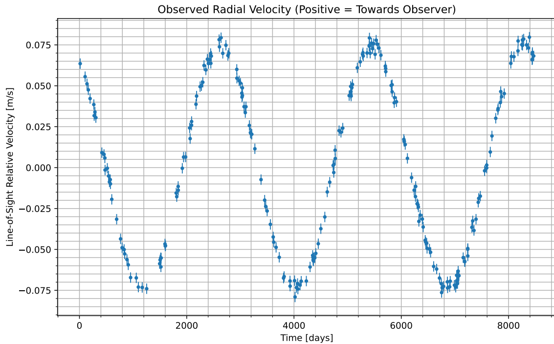
Figure 1: We have isolated the radial velocity of the host star due to the candidate planet. Data begins at UTC 2050-05-22/09:58. Positive values indicate the velocity at which the star is moving towards us; negative indicate the velocity at which it is moving away.
