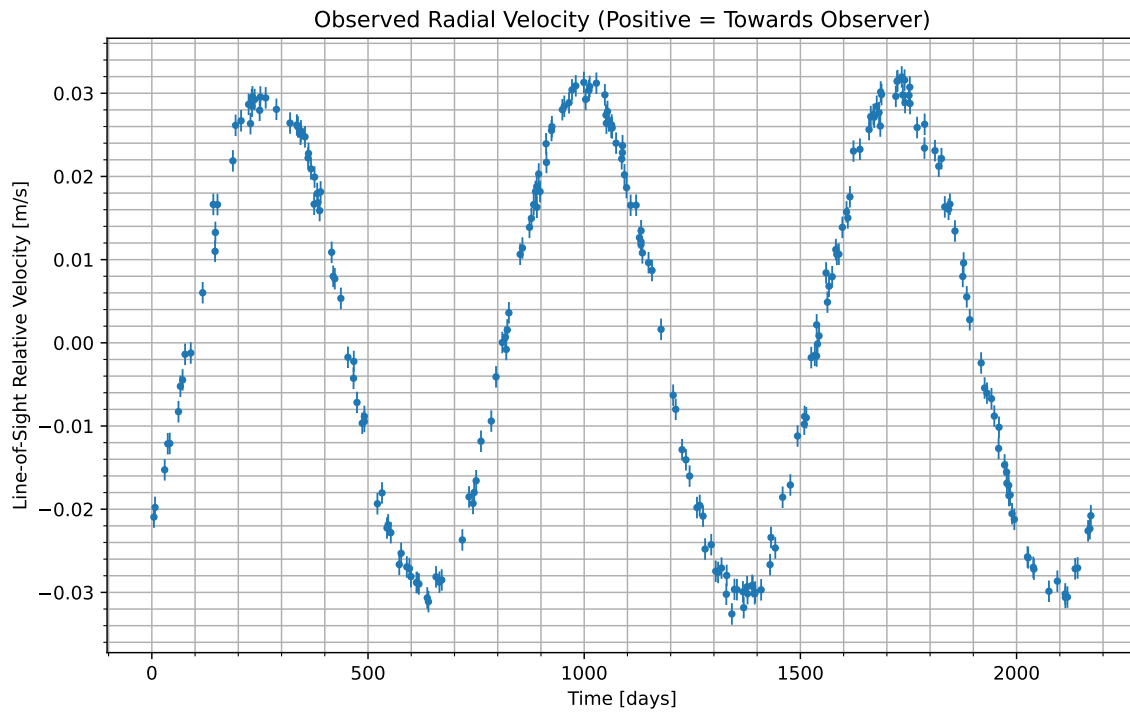
Figure 1: We have isolated the radial velocity of the host star due to the candidate planet. Data begins at UTC 2089-04-22/14:22. Positive values indicate the velocity at which the star is moving towards us; negative indicate the velocity at which it is moving away.
