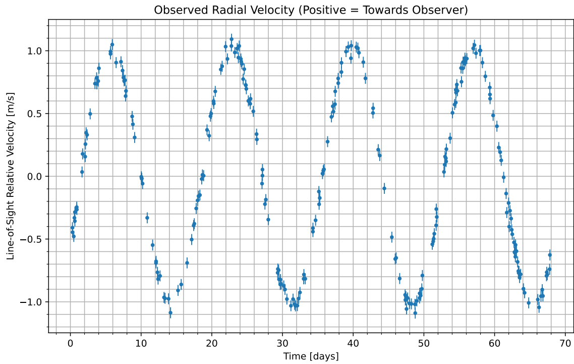
Figure 1: We have isolated the radial velocity of the host star due to the candidate planet. Data begins at UTC 2084-01-05/00:38. Positive values indicate the velocity at which the star is moving towards us; negative indicate the velocity at which it is moving away.
