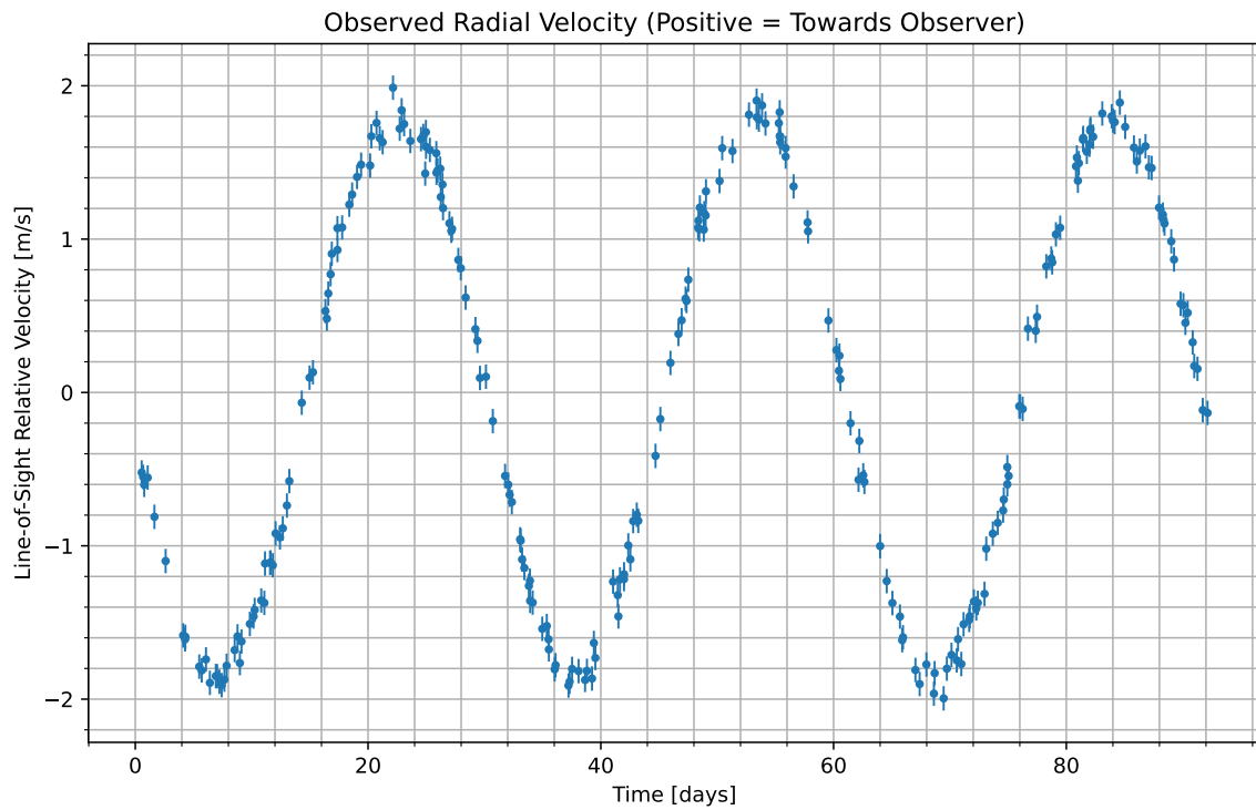
Figure 1: We have isolated the radial velocity of the host star due to the candidate planet. Data begins at UTC 2092-06-05/21:26. Positive values indicate the velocity at which the star is moving towards us; negative indicate the velocity at which it is moving away.
