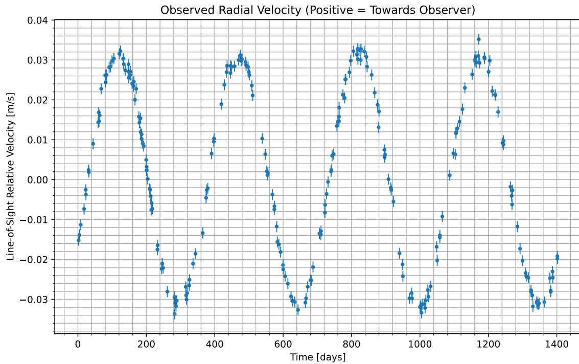
Figure 1: We have isolated the radial velocity of the host star due to the candidate planet. Data begins at UTC 2086-05-26/11:10. Positive values indicate the velocity at which the star is moving towards us; negative indicate the velocity at which it is moving away.
