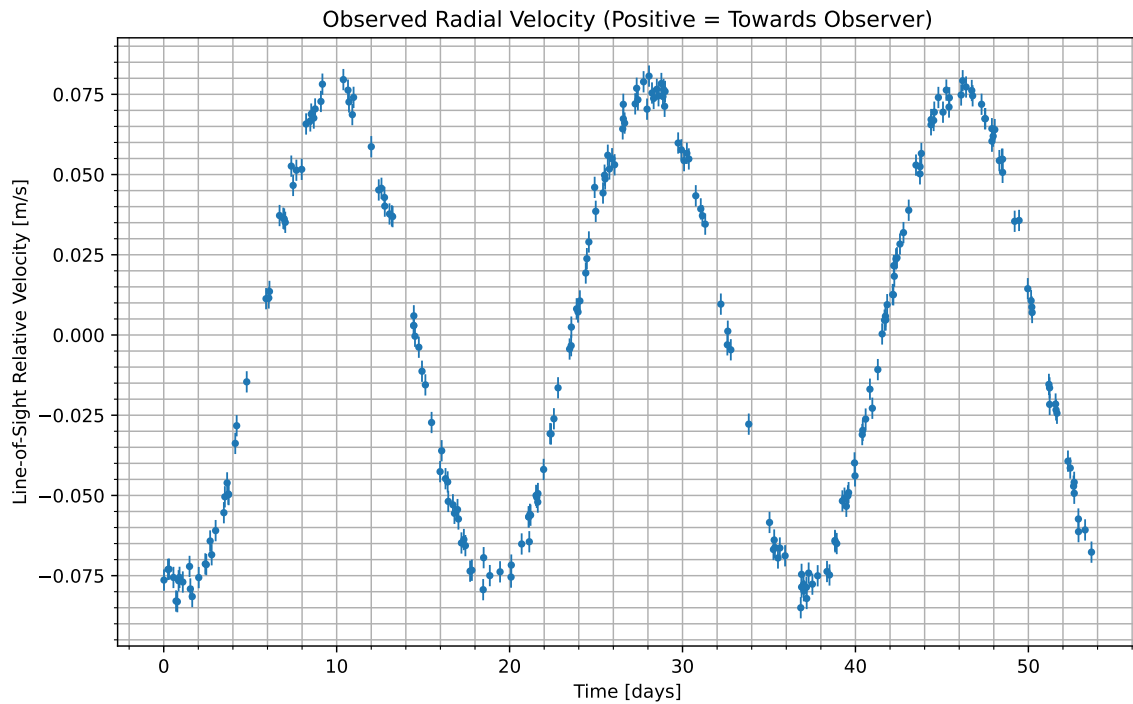
Figure 1: We have isolated the radial velocity of the host star due to the candidate planet. Data begins at UTC 2092-09-02/10:46. Positive values indicate the velocity at which the star is moving towards us; negative indicate the velocity at which it is moving away.
