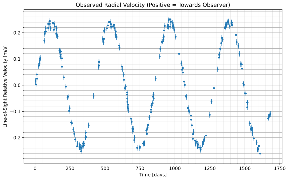
Figure 1: We have isolated the radial velocity of the host star due to the candidate planet. Data begins at UTC 2080-06-29/14:28. Positive values indicate the velocity at which the star is moving towards us; negative indicate the velocity at which it is moving away.
