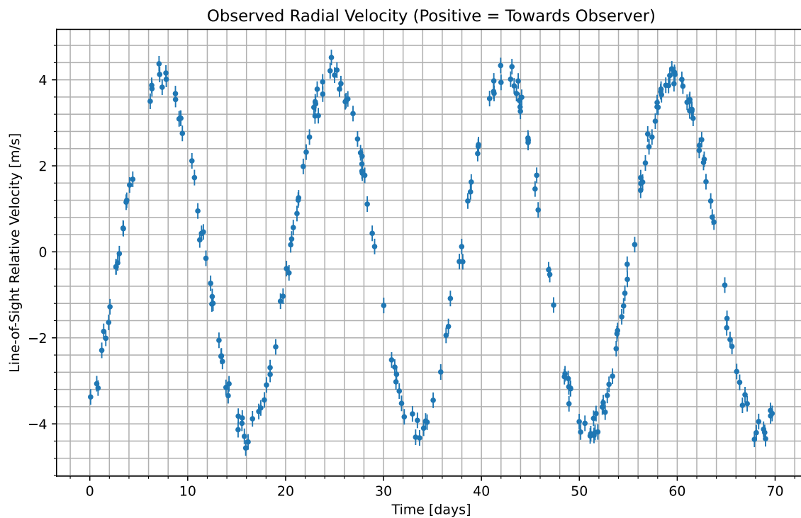
Figure 1: We have isolated the radial velocity of the host star due to the candidate planet. Data begins at UTC 2082-07-09/03:14. Positive values indicate the velocity at which the star is moving towards us; negative indicate the velocity at which it is moving away.
