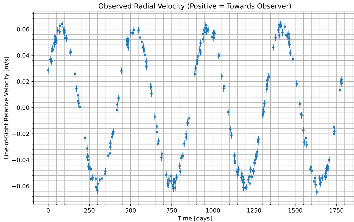
Figure 1: We have isolated the radial velocity of the host star due to the candidate planet. Data begins at UTC 2080-10-12/18:56. Positive values indicate the velocity at which the star is moving towards us; negative indicate the velocity at which it is moving away.
