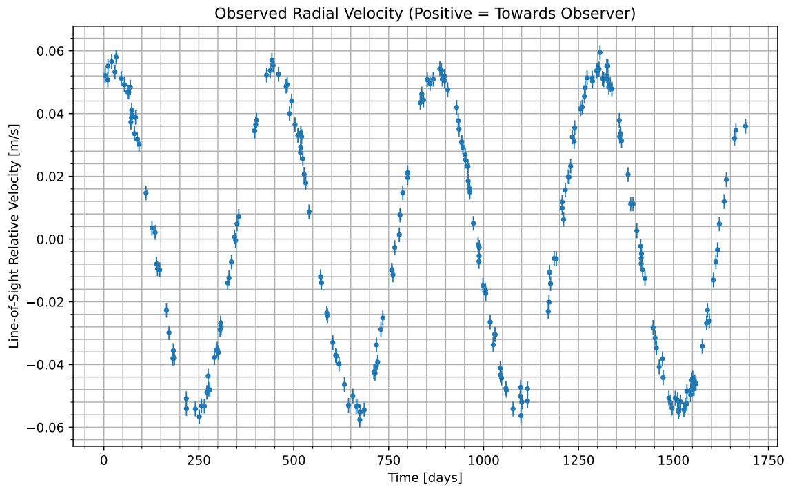
Figure 1: We have isolated the radial velocity of the host star due to the candidate planet. Data begins at UTC 2095-04-10/13:00. Positive values indicate the velocity at which the star is moving towards us; negative indicate the velocity at which it is moving away.
