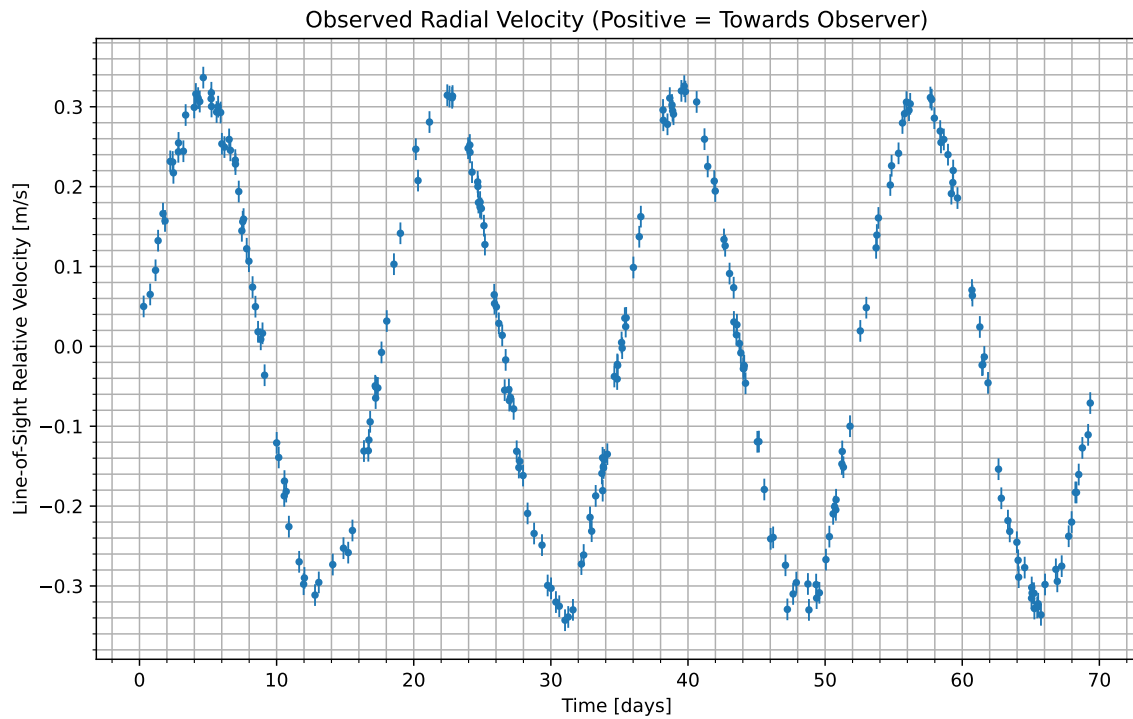
Figure 1: We have isolated the radial velocity of the host star due to the candidate planet. Data begins at UTC 2082-05-25/14:04. Positive values indicate the velocity at which the star is moving towards us; negative indicate the velocity at which it is moving away.
