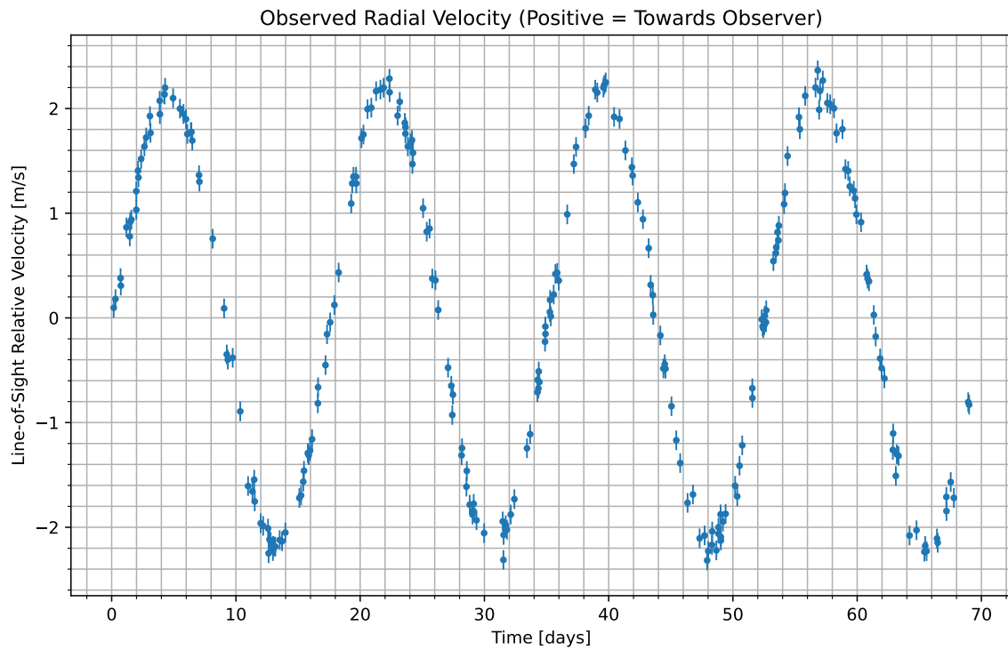
Figure 1: We have isolated the radial velocity of the host star due to the candidate planet. Data begins at UTC 2071-01-21/21:33. Positive values indicate the velocity at which the star is moving towards us; negative indicate the velocity at which it is moving away.
