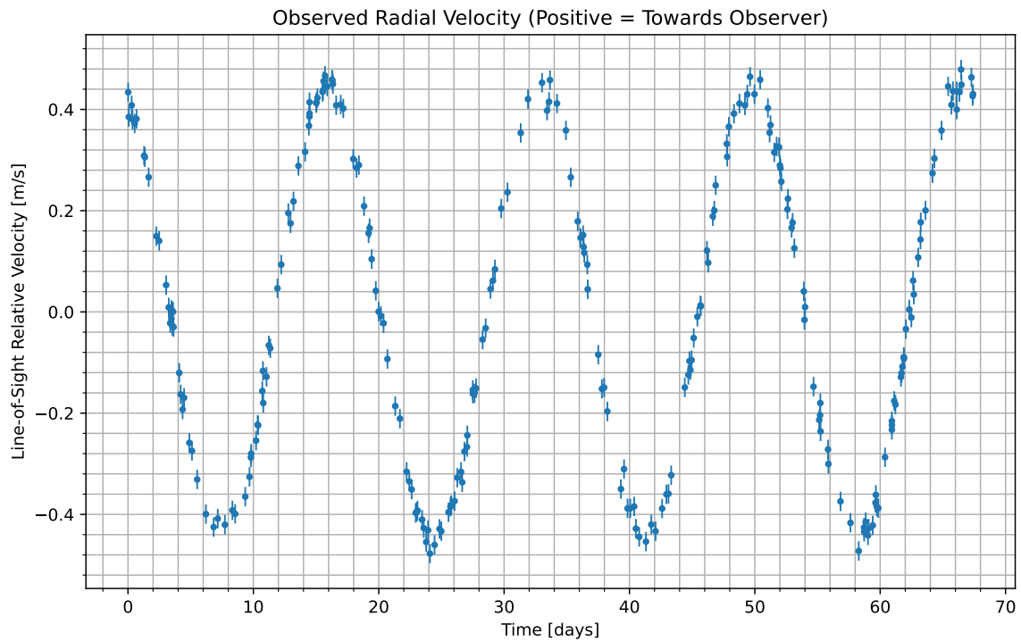
Figure 1: We have isolated the radial velocity of the host star due to the candidate planet. Data begins at UTC 2070-08-12/07:56. Positive values indicate the velocity at which the star is moving towards us; negative indicate the velocity at which it is moving away.
