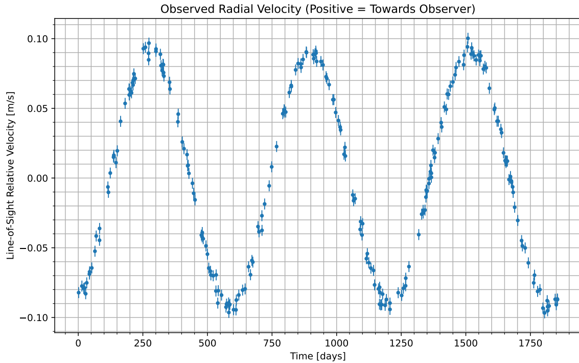
Figure 1: We have isolated the radial velocity of the host star due to the candidate planet. Data begins at UTC 2071-11-01/10:59. Positive values indicate the velocity at which the star is moving towards us; negative indicate the velocity at which it is moving away.
