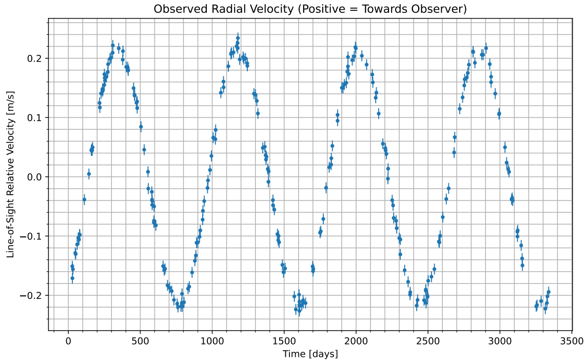
Figure 1: We have isolated the radial velocity of the host star due to the candidate planet. Data begins at UTC 2080-10-11/07:30. Positive values indicate the velocity at which the star is moving towards us; negative indicate the velocity at which it is moving away.
