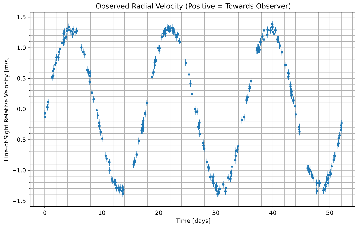
Figure 1: We have isolated the radial velocity of the host star due to the candidate planet. Data begins at UTC 2076-05-11/07:22. Positive values indicate the velocity at which the star is moving towards us; negative indicate the velocity at which it is moving away.
