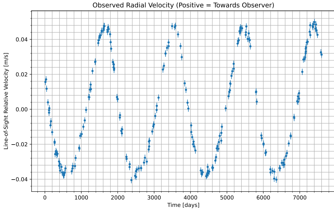
Figure 1: We have isolated the radial velocity of the host star due to the candidate planet. Data begins at UTC 2069-02-09/05:36. Positive values indicate the velocity at which the star is moving towards us; negative indicate the velocity at which it is moving away.
