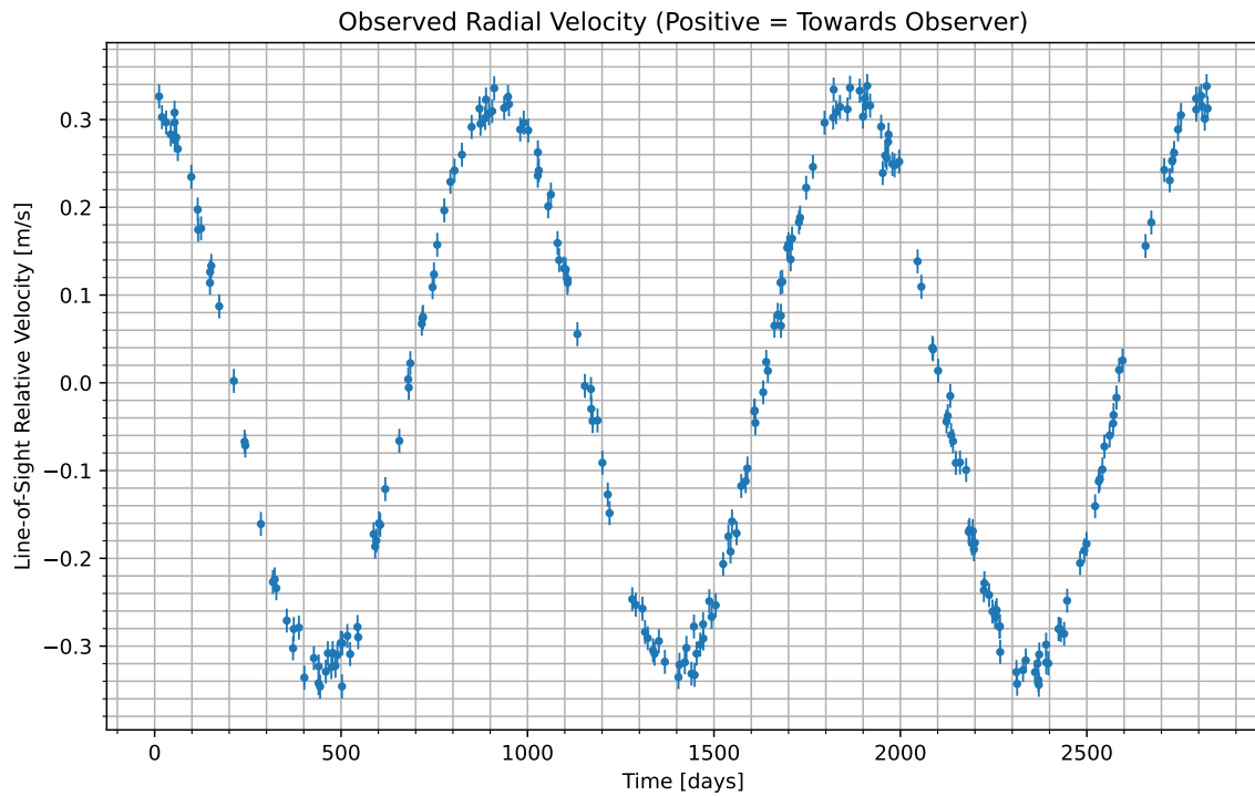
Figure 1: We have isolated the radial velocity of the host star due to the candidate planet. Data begins at UTC 2062-08-10/13:21. Positive values indicate the velocity at which the star is moving towards us; negative indicate the velocity at which it is moving away.
