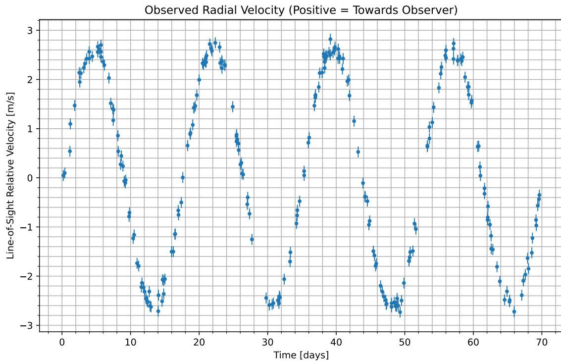
Figure 1: We have isolated the radial velocity of the host star due to the candidate planet. Data begins at UTC 2076-04-27/02:54. Positive values indicate the velocity at which the star is moving towards us; negative indicate the velocity at which it is moving away.
