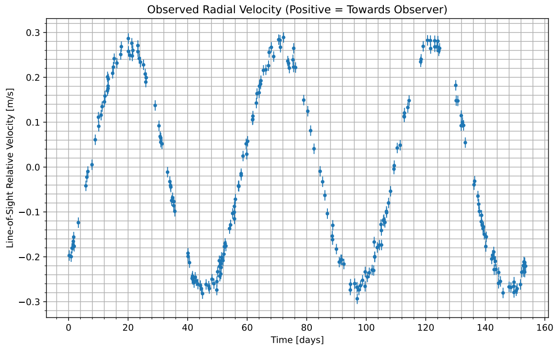
Figure 1: We have isolated the radial velocity of the host star due to the candidate planet. Data begins at UTC 2080-05-03/04:43. Positive values indicate the velocity at which the star is moving towards us; negative indicate the velocity at which it is moving away.
