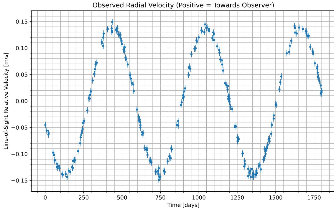
Figure 1: We have isolated the radial velocity of the host star due to the candidate planet. Data begins at UTC 2073-03-10/19:05. Positive values indicate the velocity at which the star is moving towards us; negative indicate the velocity at which it is moving away.
