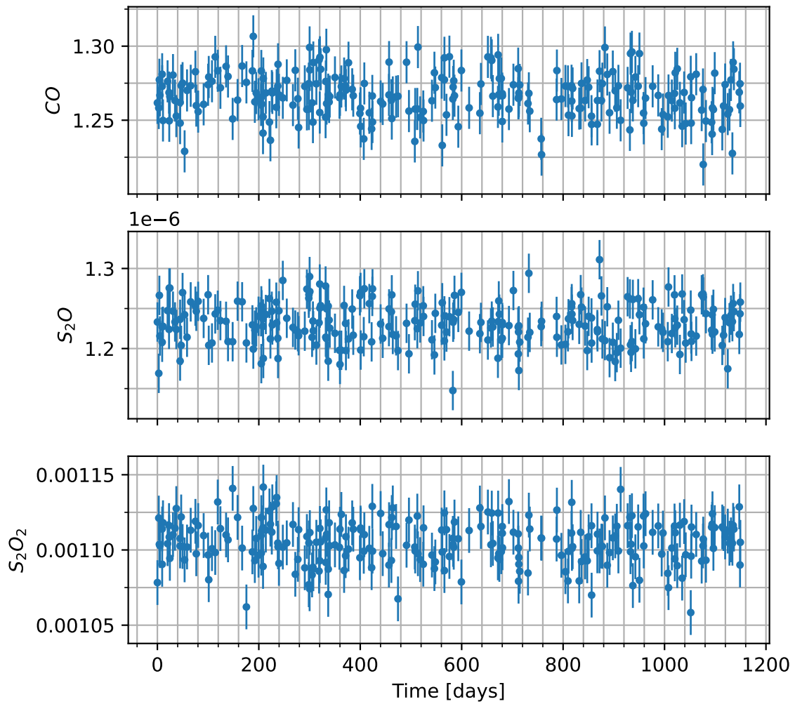
Figure 4: Concentration of various additional gases in the atmosphere of the candidate planet versus time. Note that the y-axis will usually only show the variation multiplied by some factor, shown in the upper left, and then added to some normal amount, also in the upper-left.
