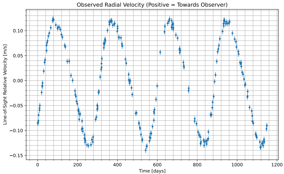
Figure 1: We have isolated the radial velocity of the host star due to the candidate planet. Data begins at UTC 2092-12-18/20:04. Positive values indicate the velocity at which the star is moving towards us; negative indicate the velocity at which it is moving away.
