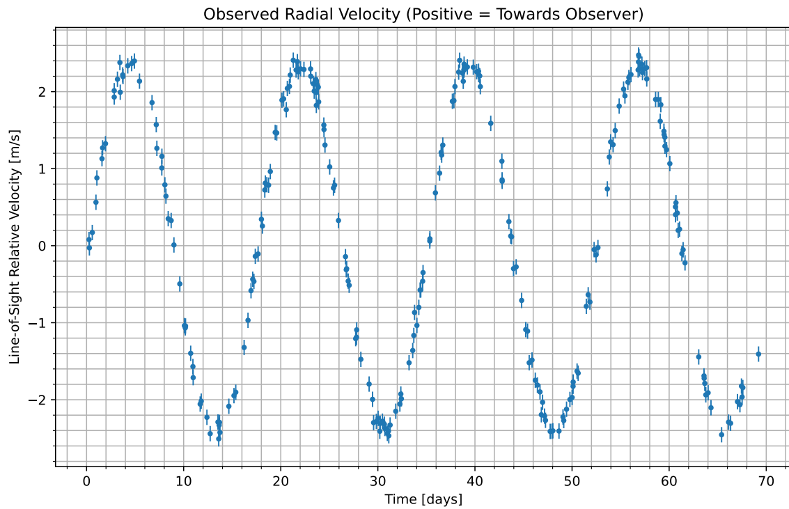
Figure 1: We have isolated the radial velocity of the host star due to the candidate planet. Data begins at UTC 2077-09-09/18:32. Positive values indicate the velocity at which the star is moving towards us; negative indicate the velocity at which it is moving away.
