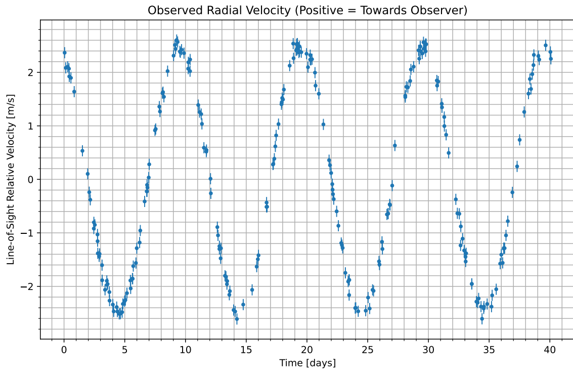
Figure 1: We have isolated the radial velocity of the host star due to the candidate planet. Data begins at UTC 2081-04-20/21:37. Positive values indicate the velocity at which the star is moving towards us; negative indicate the velocity at which it is moving away.
