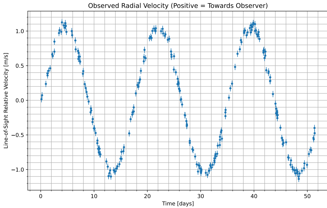
Figure 1: We have isolated the radial velocity of the host star due to the candidate planet. Data begins at UTC 2078-08-20/21:39. Positive values indicate the velocity at which the star is moving towards us; negative indicate the velocity at which it is moving away.
