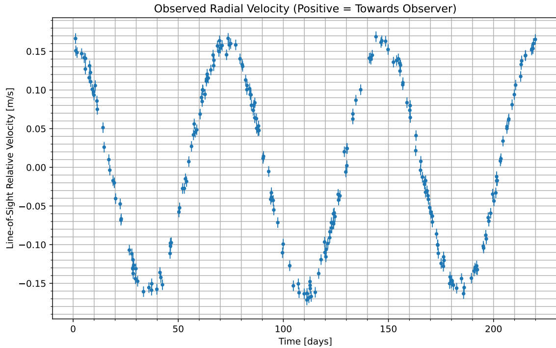
Figure 1: We have isolated the radial velocity of the host star due to the candidate planet. Data begins at UTC 2074-06-17/13:12. Positive values indicate the velocity at which the star is moving towards us; negative indicate the velocity at which it is moving away.
