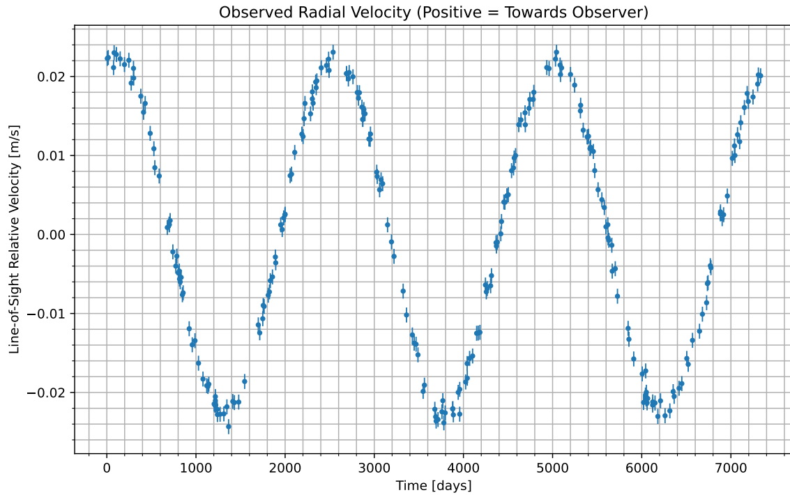
Figure 1: We have isolated the radial velocity of the host star due to the candidate planet. Data begins at UTC 2080-09-04/04:25. Positive values indicate the velocity at which the star is moving towards us; negative indicate the velocity at which it is moving away.
