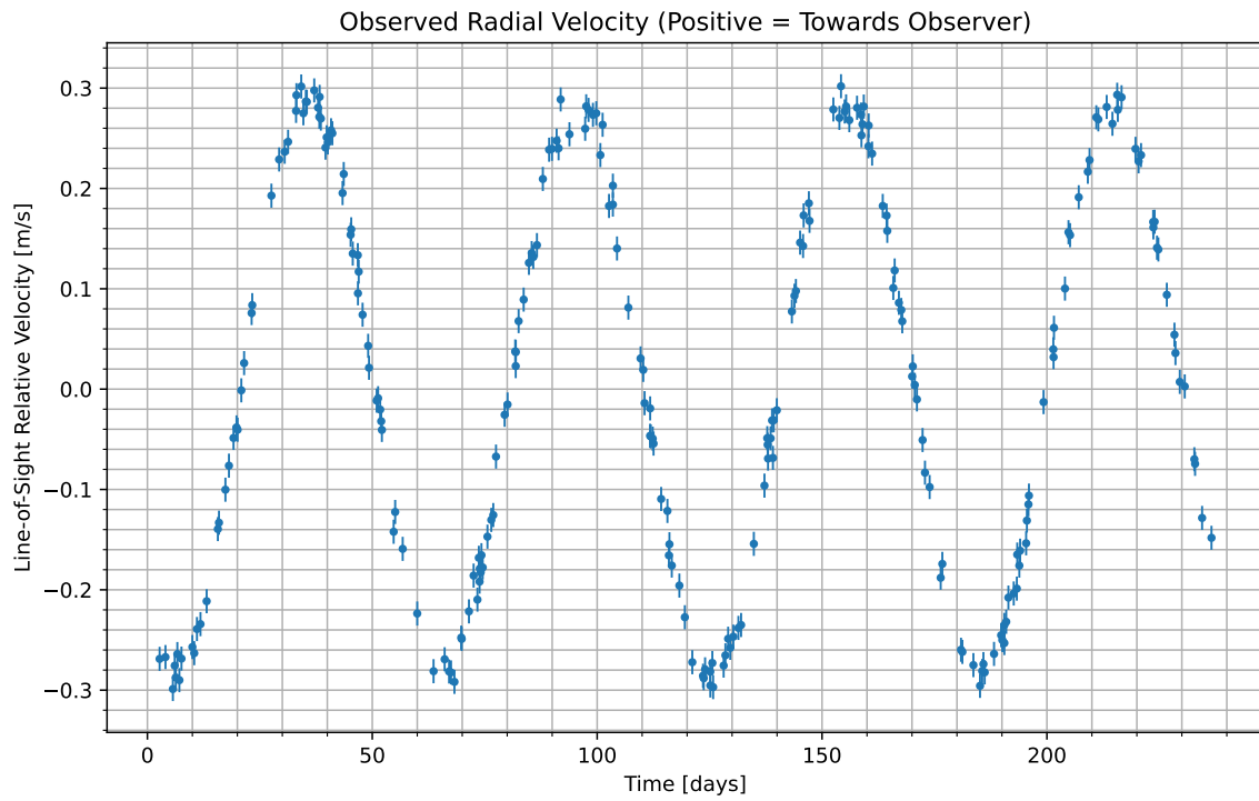
Figure 1: We have isolated the radial velocity of the host star due to the candidate planet. Data begins at UTC 2075-09-09/09:06. Positive values indicate the velocity at which the star is moving towards us; negative indicate the velocity at which it is moving away.
