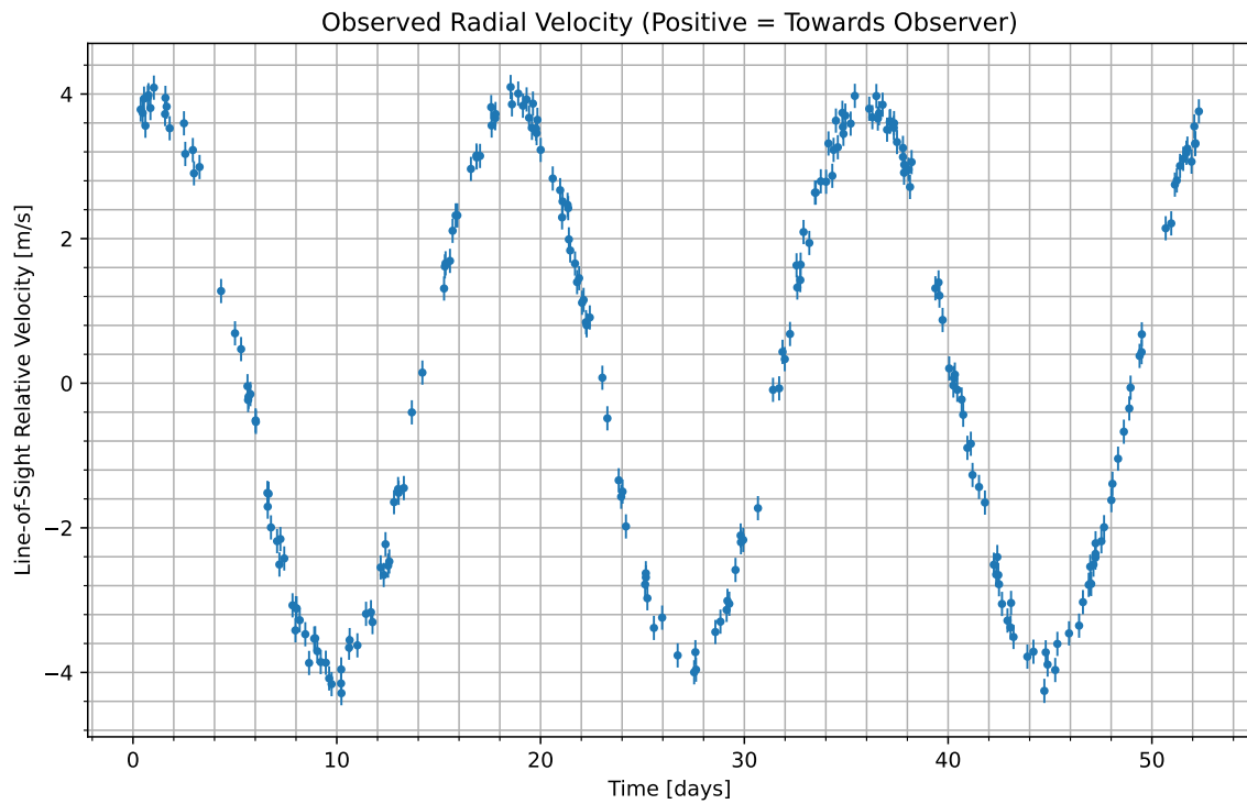
Figure 1: We have isolated the radial velocity of the host star due to the candidate planet. Data begins at UTC 2083-09-03/07:09. Positive values indicate the velocity at which the star is moving towards us; negative indicate the velocity at which it is moving away.
