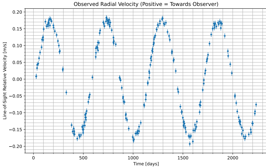
Figure 1: We have isolated the radial velocity of the host star due to the candidate planet. Data begins at UTC 2083-08-23/16:57. Positive values indicate the velocity at which the star is moving towards us; negative indicate the velocity at which it is moving away.
