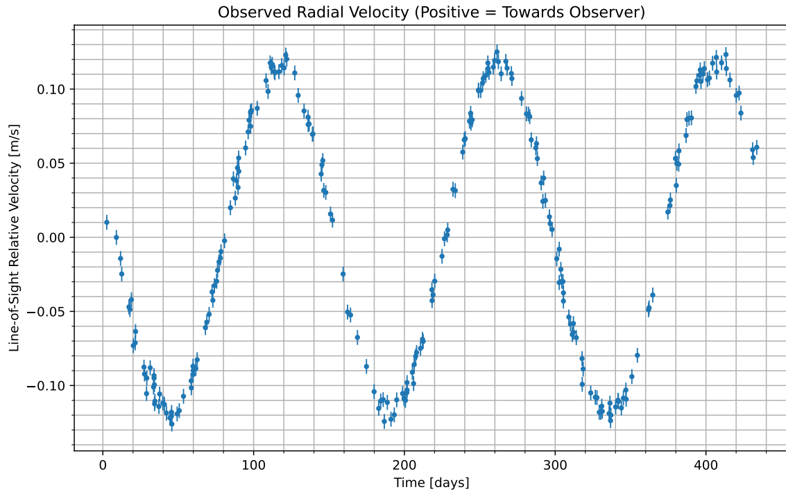
Figure 1: We have isolated the radial velocity of the host star due to the candidate planet. Data begins at UTC 2074-04-11/08:08. Positive values indicate the velocity at which the star is moving towards us; negative indicate the velocity at which it is moving away.
