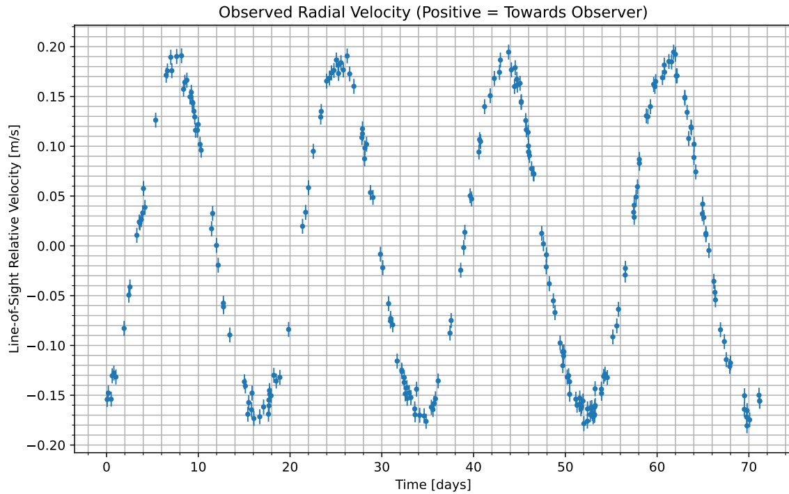
Figure 1: We have isolated the radial velocity of the host star due to the candidate planet. Data begins at UTC 2070-12-19/04:33. Positive values indicate the velocity at which the star is moving towards us; negative indicate the velocity at which it is moving away.
