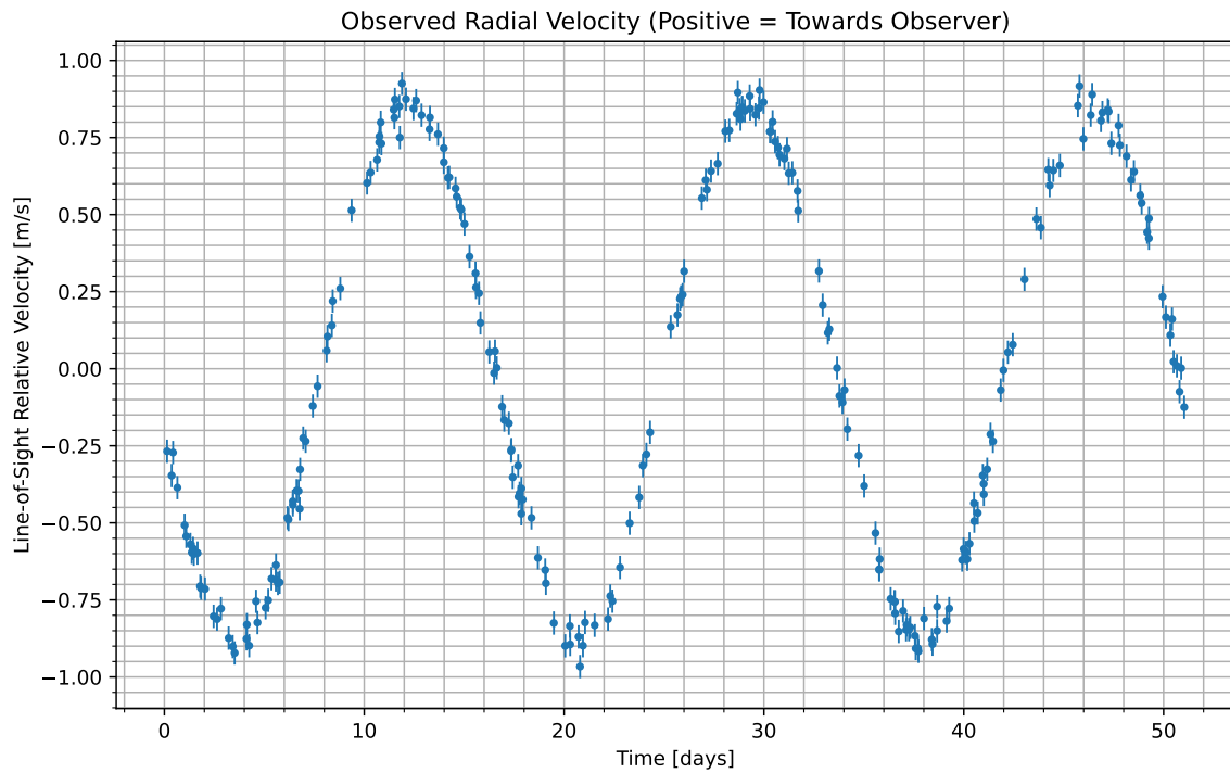
Figure 1: We have isolated the radial velocity of the host star due to the candidate planet. Data begins at UTC 2094-11-21/20:31. Positive values indicate the velocity at which the star is moving towards us; negative indicate the velocity at which it is moving away.
