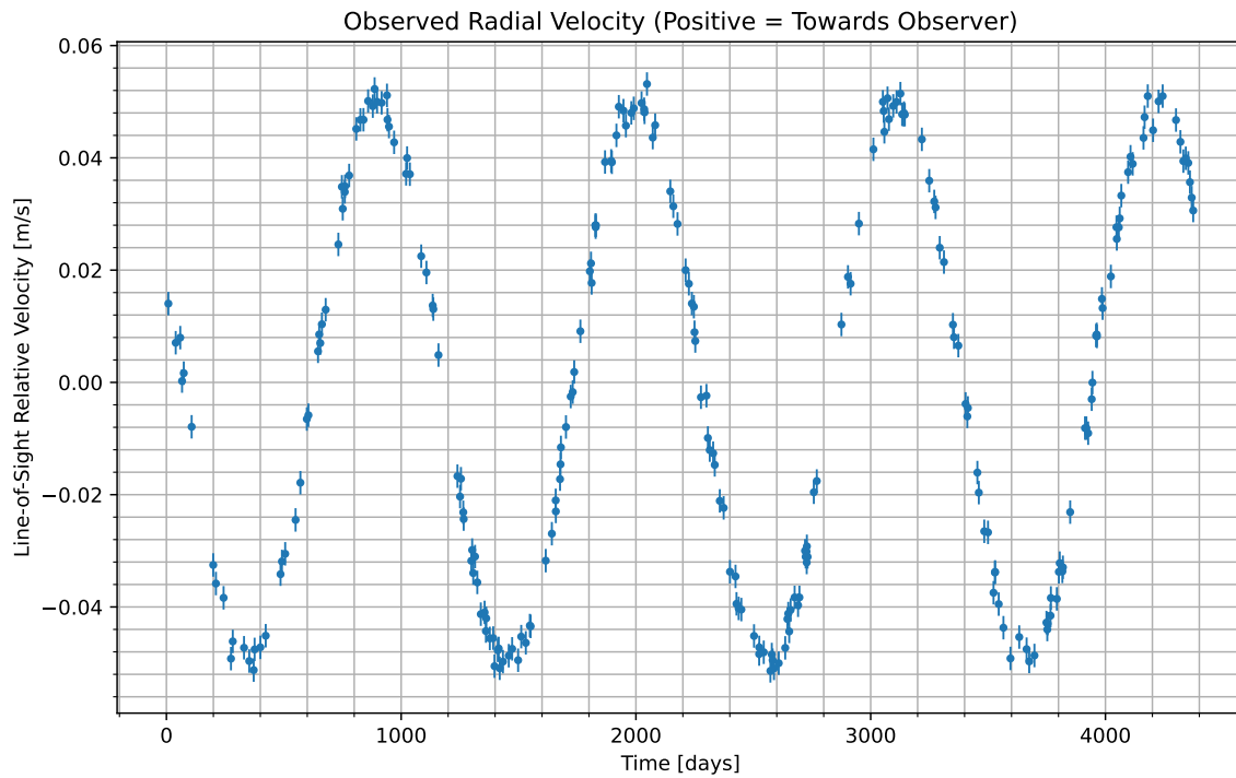
Figure 1: We have isolated the radial velocity of the host star due to the candidate planet. Data begins at UTC 2070-05-03/20:36. Positive values indicate the velocity at which the star is moving towards us; negative indicate the velocity at which it is moving away.
