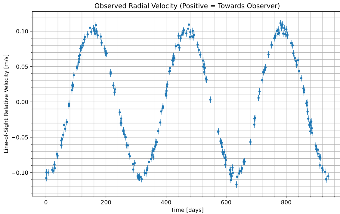
Figure 1: We have isolated the radial velocity of the host star due to the candidate planet. Data begins at UTC 2088-06-25/15:00. Positive values indicate the velocity at which the star is moving towards us; negative indicate the velocity at which it is moving away.
