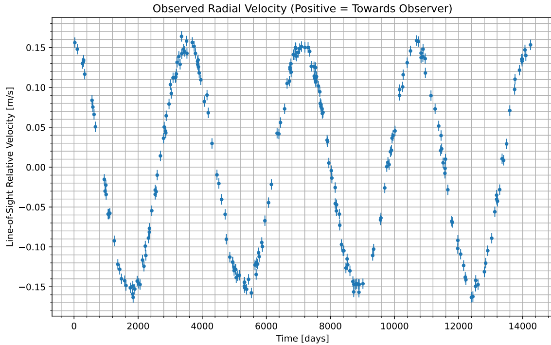
Figure 1: We have isolated the radial velocity of the host star due to the candidate planet. Data begins at UTC 2049-03-20/08:18. Positive values indicate the velocity at which the star is moving towards us; negative indicate the velocity at which it is moving away.
