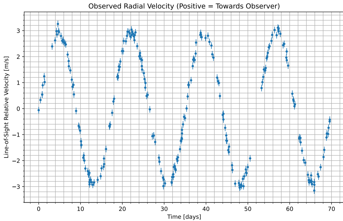
Figure 1: We have isolated the radial velocity of the host star due to the candidate planet. Data begins at UTC 2073-11-09/12:56. Positive values indicate the velocity at which the star is moving towards us; negative indicate the velocity at which it is moving away.
