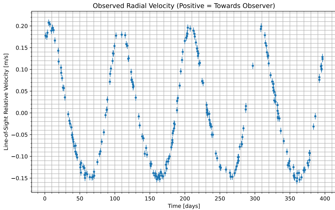
Figure 1: We have isolated the radial velocity of the host star due to the candidate planet. Data begins at UTC 2080-06-06/09:02. Positive values indicate the velocity at which the star is moving towards us; negative indicate the velocity at which it is moving away.
